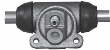
894930 Wheel Cylinder Asm Cushman Haulster/Truckster 1996 - Current
